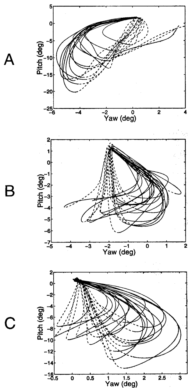
Figure 6. Pitch versus yaw angle in mastication. The figure shows bilateral chewing, normal bolus size—octopus, celery, steak, and peanuts. Panel A is DO, B is AL, and C is MT. Opening (dashed lines) and closing movements (solid lines) are shown.
